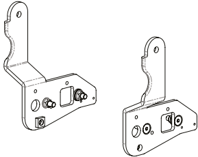
Seat bracket Kserie BeGe 7000/9000 TJ LH+RH 800101
