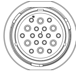
C6 CONNECTON
